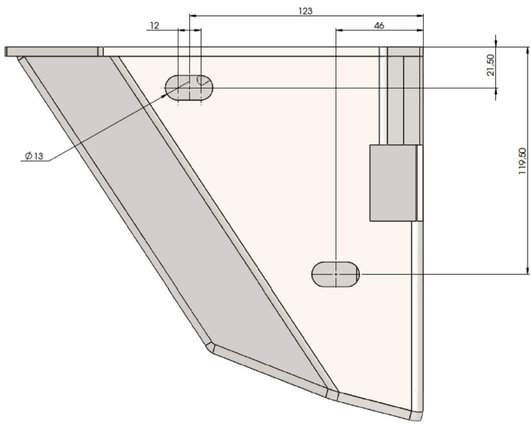
Mounting holes: dimensions in mm
